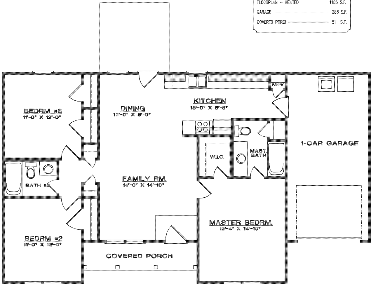
FLOORPLAN
